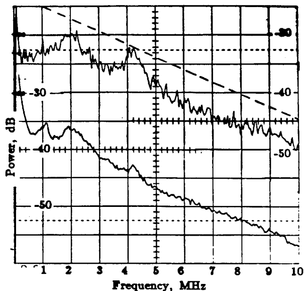
Figure 2. Spectra from the BPM at the output of Tank 7 for high (top) and for low (bottom) pressure in the 750 keV injection line; the dashed line is the response of the RF detector, -20 dB/octave.
