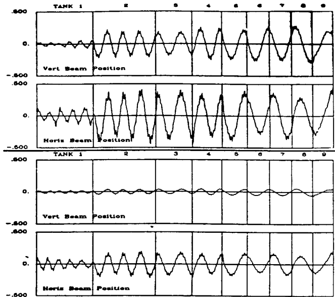
Figure 4. Parmila predictions of beam positions down the Linac resulting from slight 750 keV offset.
