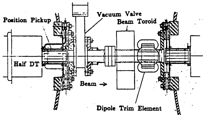
Figure 1. FNAL Linac BPM assembly drawing.
