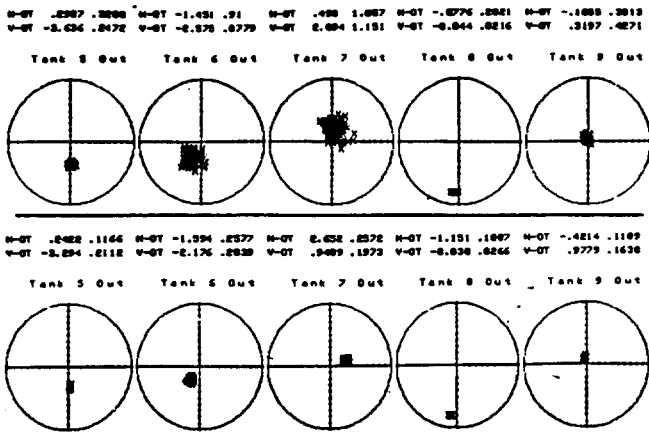
Figure 3. "Bull's eye" plots of beam positions through the Linac, high pressure in injection line, before (top) and after (bottom) Parmila -directed quad tuning.
